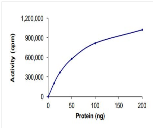
Functional Studies - Recombinant human Chk1 protein (ab60762)
