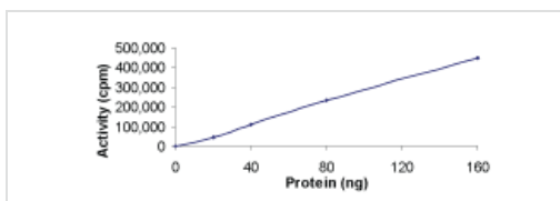
Functional Studies - Recombinant human Chk1 protein (ab60762)
