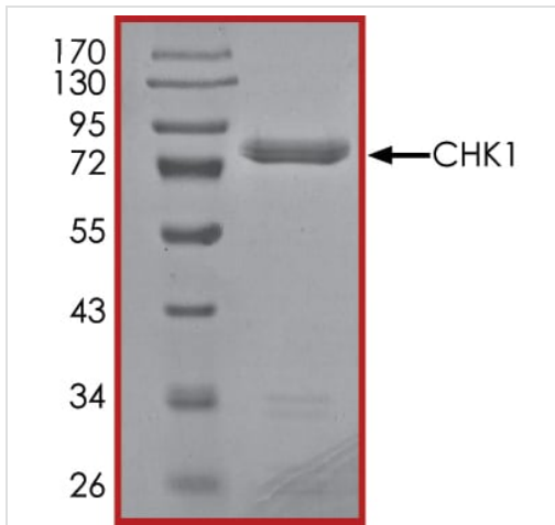
SDS-PAGE - Recombinant human Chk1 protein (ab60762)
