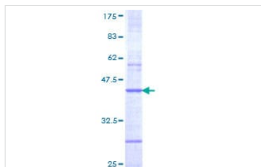
ab158120 on a 12.5% SDS-PAGE stained with Coomassie Blue.
