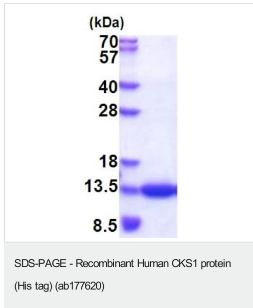
15% SDS-PAGE analysis of ab177620 (3µg)
