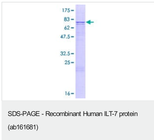
ab161681 on a 12.5% SDS-PAGE stained with Coomassie Blue.
