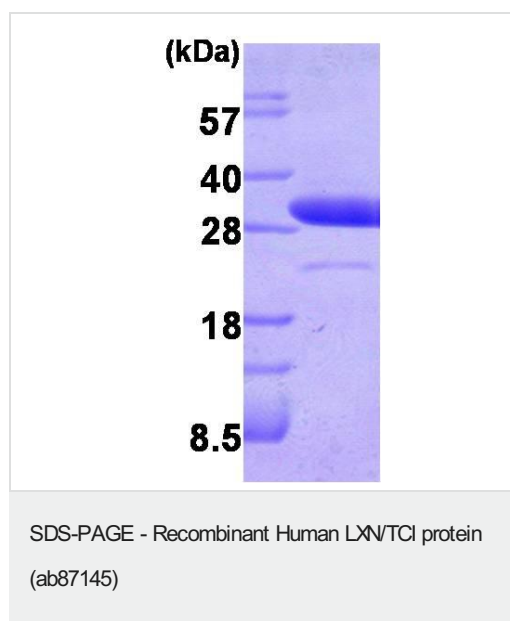
15% SDS-PAGE showing ab87145 (3ug)
