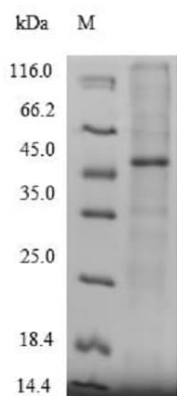
SDS-PAGE - Recombinant Human MICAL2 protein (His tag) (ab241260)
