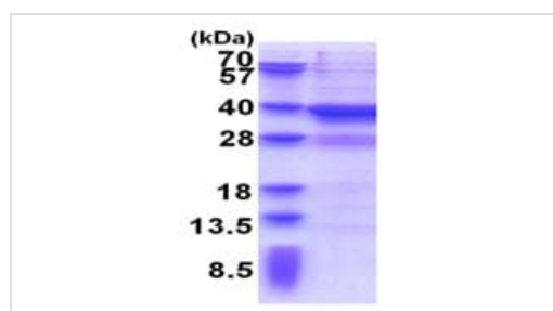
15% SDS-PAGE analysis of ab176084 (3µg).
