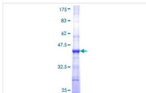
ab153539 on a 12.5% SDS-PAGE stained with Coomassie Blue.
