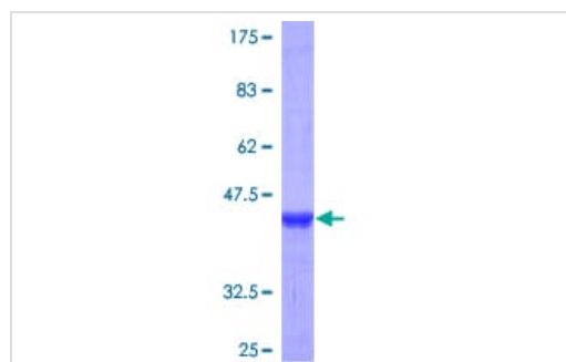
ab163637 on a 12.5% SDS-PAGE stained with Coomassie Blue.
