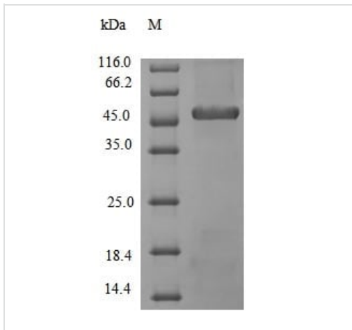
SDS-PAGE - Recombinant Human Subtilisin Carlsberg protein (Tagged) (ab237794)
