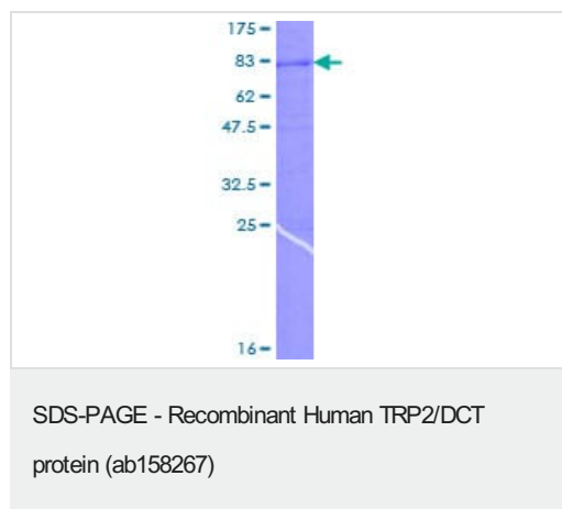
ab158267 on a 12.5% SDS-PAGE stained with Coomassie Blue.
