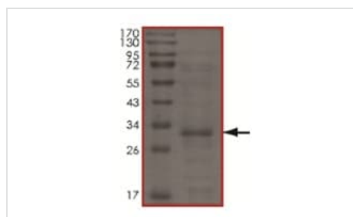
SDS Page analysis of ab167938
