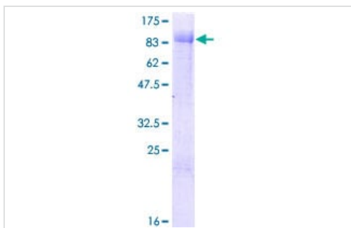
SDS-PAGE - Recombinant Human ZBTB46 protein (ab165467)
