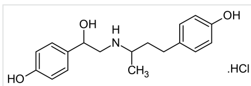
2D chemical structure image of ab142536, Ractopamine hydrochloride, beta1 and beta2-adrenoceptor agonist
