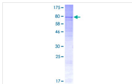
ab162666 on a 12.5% SDS-PAGE stained with Coomassie Blue.
