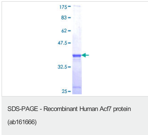
ab161666 on a 12.5% SDS-PAGE stained with Coomassie Blue.
