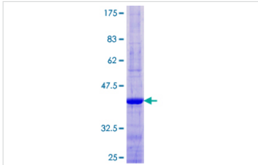
ab166289 on a 12.5% SDS-PAGE stained with Coomassie Blue.
