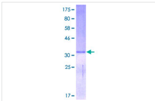
ab158273 on a 12.5% SDS-PAGE stained with Coomassie Blue.
