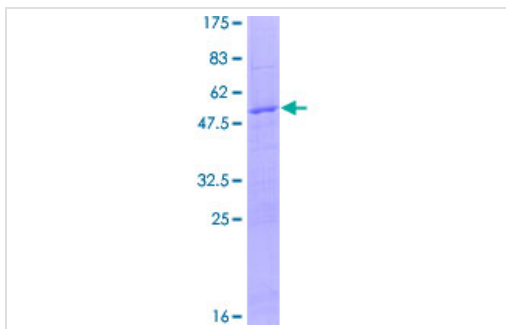
ab160711 on a 12.5% SDS-PAGE stained with Coomassie Blue.
