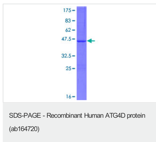
ab164720 on a 12.5% SDS-PAGE stained with Coomassie Blue.
