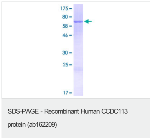
ab162209 on a 12.5% SDS-PAGE stained with Coomassie Blue.
