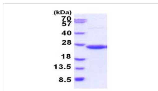
15% SDS-PAGE analysis of 3 µg of ab187438.
