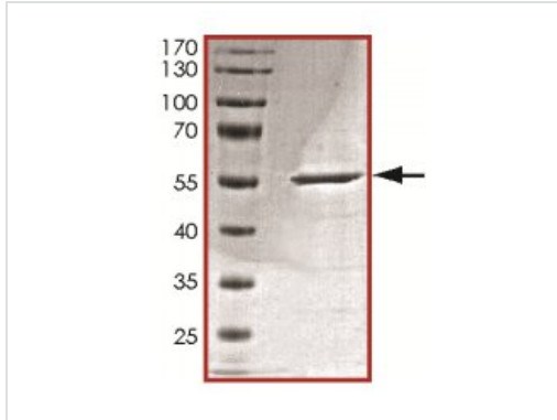
SDS-PAGE analysis of ab126917.
