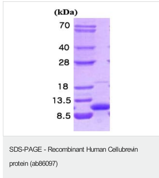
15% SDS-PAGE showing ab86097 at approximately 8.7kDa (3µg).
