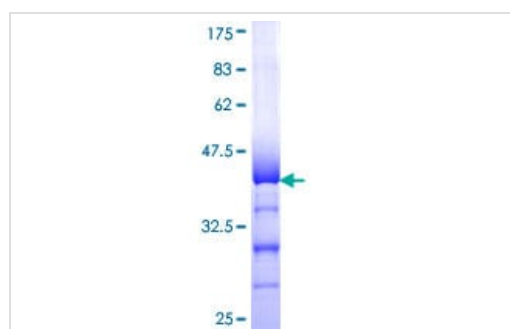
ab158335 on a 12.5% SDS-PAGE stained with Coomassie Blue.
