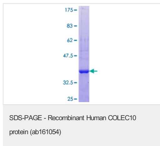
ab161054 on a 12.5% SDS-PAGE stained with Coomassie Blue.
