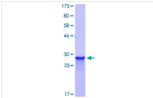
SDS-PAGE - Recombinant Human CPNE5 protein (ab163628)
