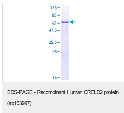
ab163997 on a 12.5% SDS-PAGE stained with Coomassie Blue.
