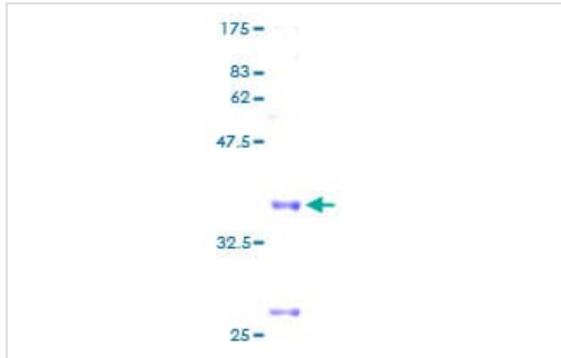
ab158177 on a 12.5% SDS-PAGE stained with Coomassie Blue.
