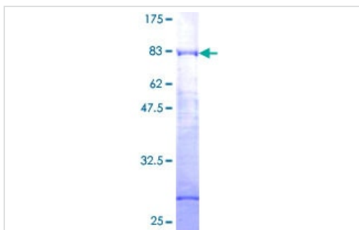
ab159327 on a 12.5% SDS-PAGE stained with Coomassie Blue.
