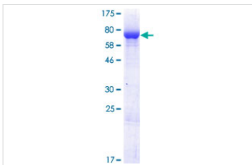
ab163785 on a 12.5% SDS-PAGE stained with Coomassie Blue.
