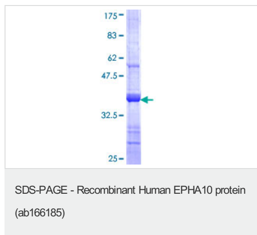
ab166185 on a 12.5% SDS-PAGE stained with Coomassie Blue.
