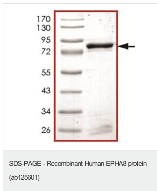
SDS Page analysis of ab125601
