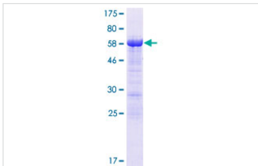
ab165105 on a 12.5% SDS-PAGE stained with Coomassie Blue.
