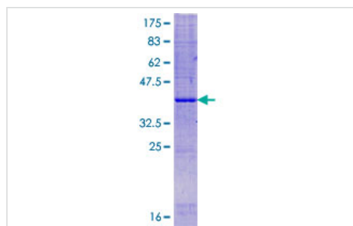
SDS-PAGE - Recombinant Human FAM19A4 protein (ab165632)
