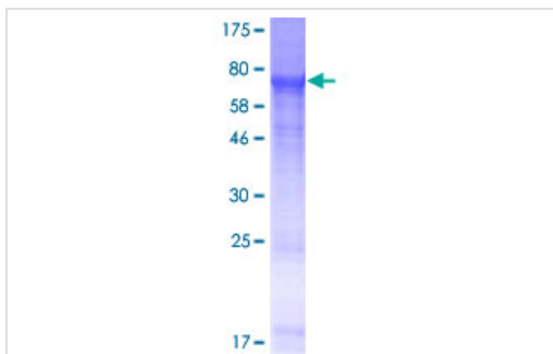
ab163140 on a 12.5% SDS-PAGE stained with Coomassie Blue.
