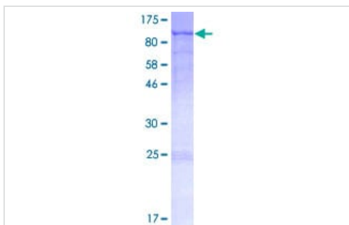
ab166266 on a 12.5% SDS-PAGE stained with Coomassie Blue.
