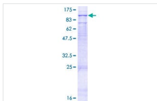
12.5% SDS-PAGE analysis of ab132334 stained with Coomassie Blue.
