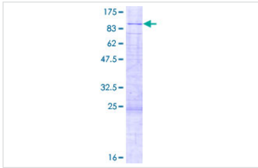
SDS-PAGE - Recombinant Human FTSJ3 protein (ab165132)
