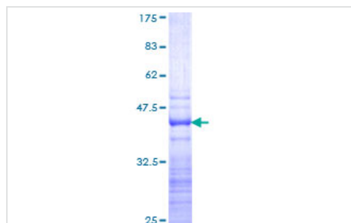
SDS-PAGE - Recombinant Human GA2L2 protein (ab166010)
