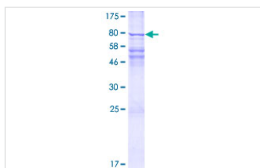
ab158516 on a 12.5% SDS-PAGE stained with Coomassie Blue.
