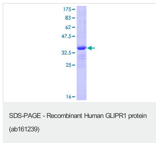
ab161239 on a 12.5% SDS-PAGE stained with Coomassie Blue.
