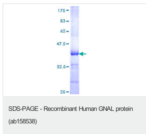
ab158538 on a 12.5% SDS-PAGE stained with Coomassie Blue.
