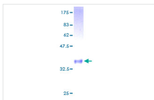
ab158543 on a 12.5% SDS-PAGE stained with Coomassie Blue.
