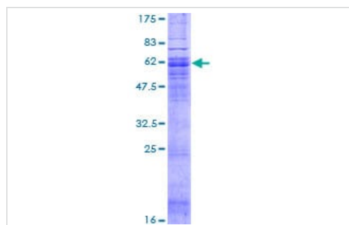
ab153291 on a 12.5% SDS-PAGE stained with Coomassie Blue.
