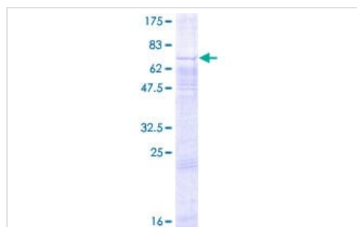
ab158568 on a 12.5% SDS-PAGE stained with Coomassie Blue.
