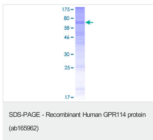
ab165962 on a 12.5% SDS-PAGE stained with Coomassie Blue.
