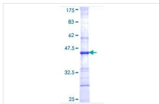
SDS-PAGE - Recombinant Human GST-1 protein (ab152884)
