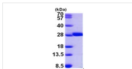
SDS-PAGE - Recombinant Human GSTM2 protein (ab99435)
