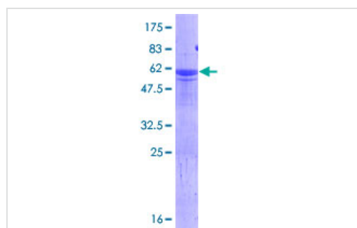
ab132389 on 12.5% SDS-PAGE stained with Coomassie Blue.
